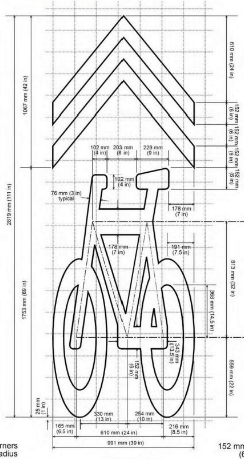
Figure 9C-104 (CA). Shared Roadway Bicycle Marking
