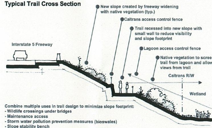
Typical Trail Cross Section
